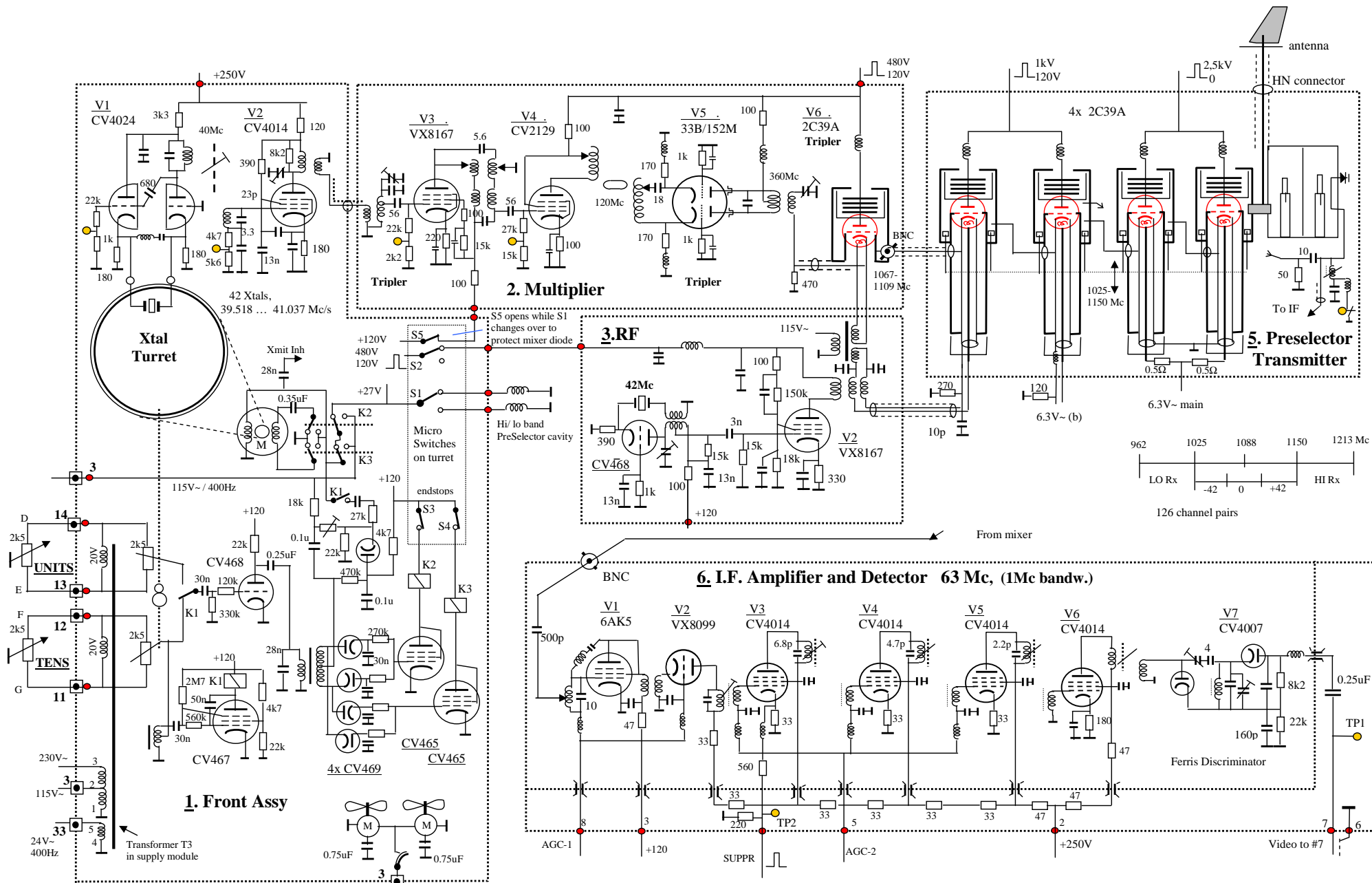
STARN-21 RF modules 11 June 2007
