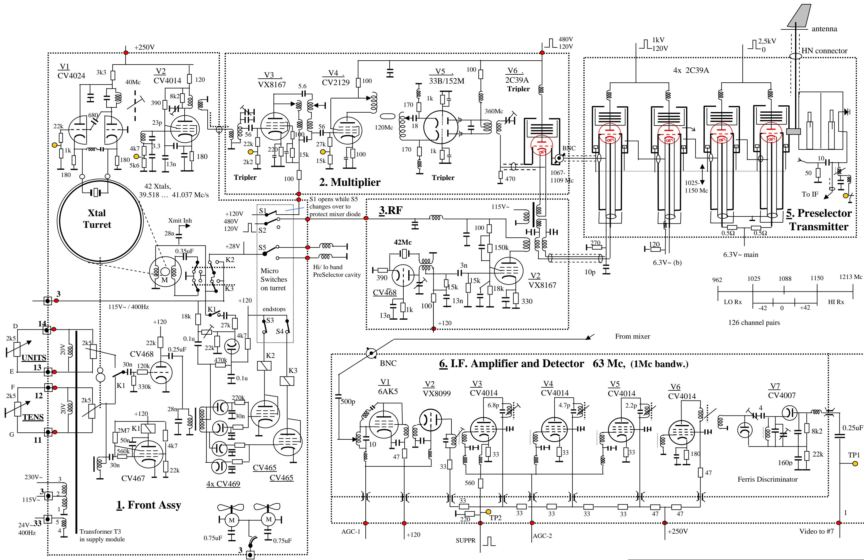
STARN-21 RF modules 11 june 2007
