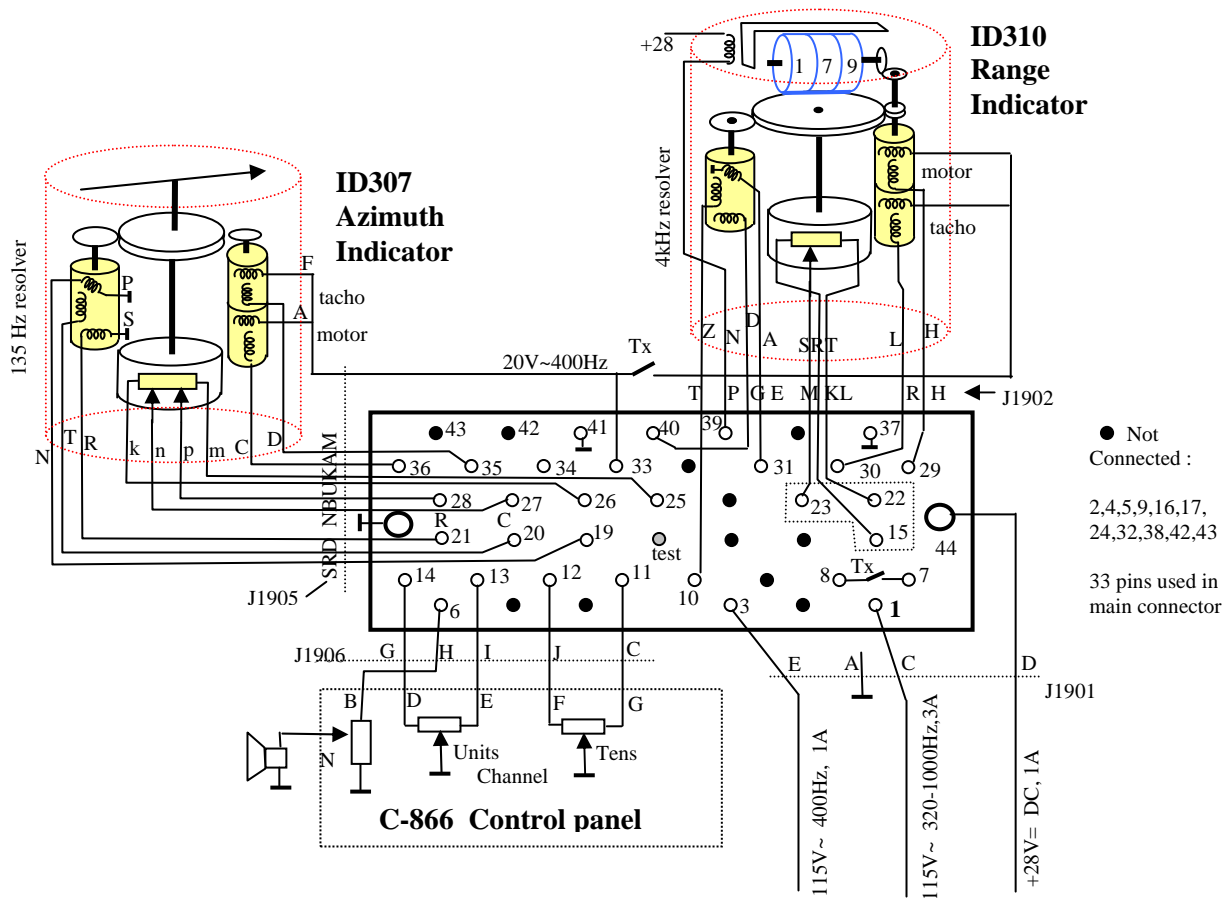
STARN-21 Power Supply and interface June 2007
