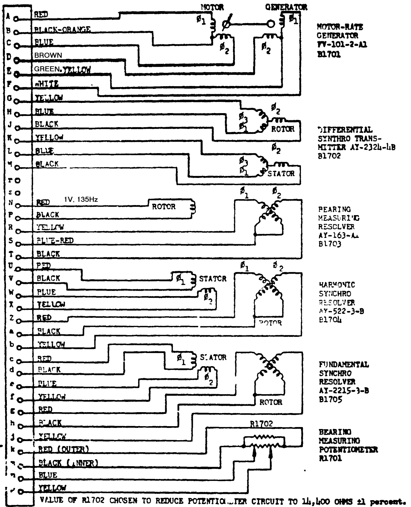
FIGURE 2. Schematic, ID-307/ARN; indicator, azimuth
