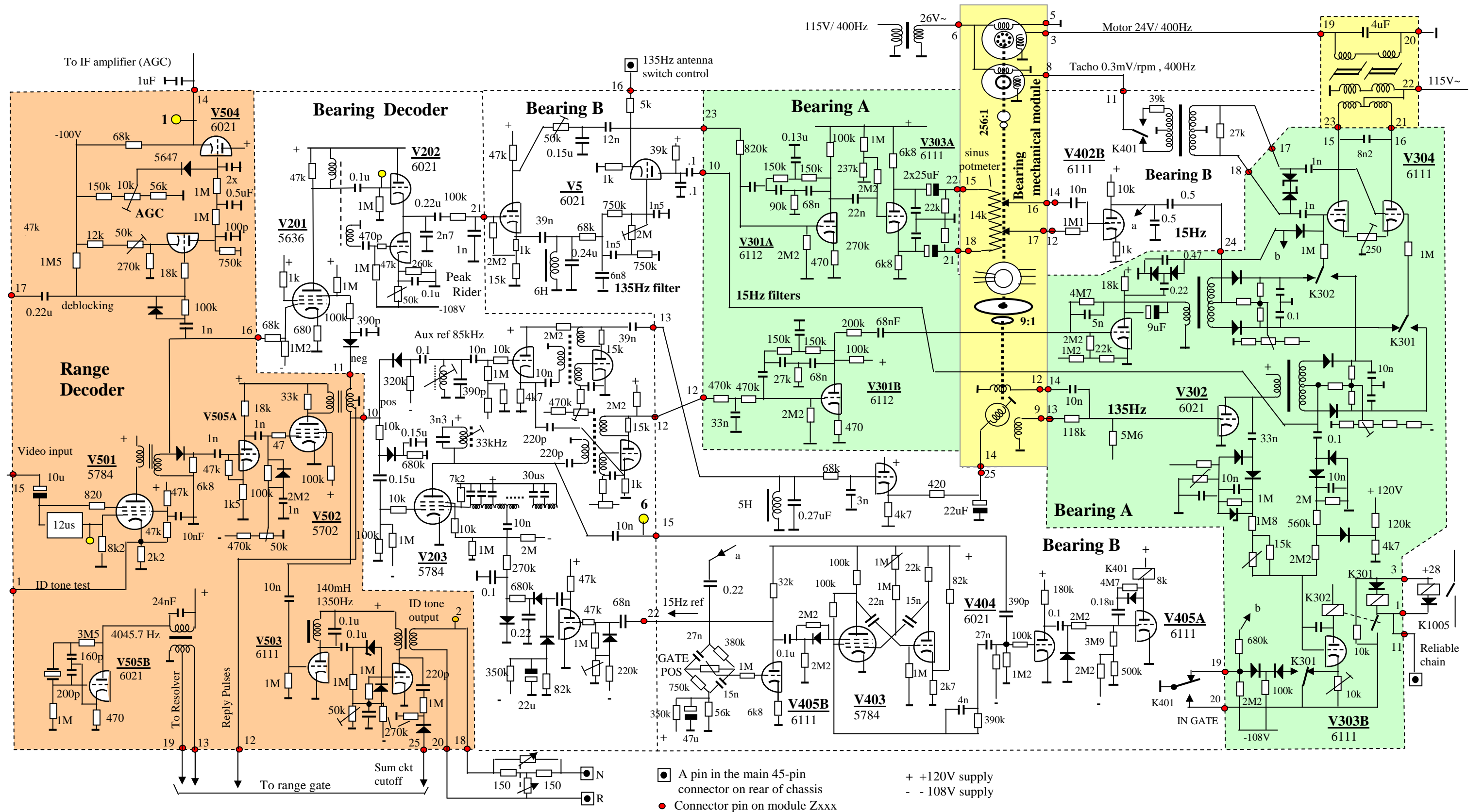
ARN52 Video and Azimuth Circuit Diagram 13 Dec 2010 KB
