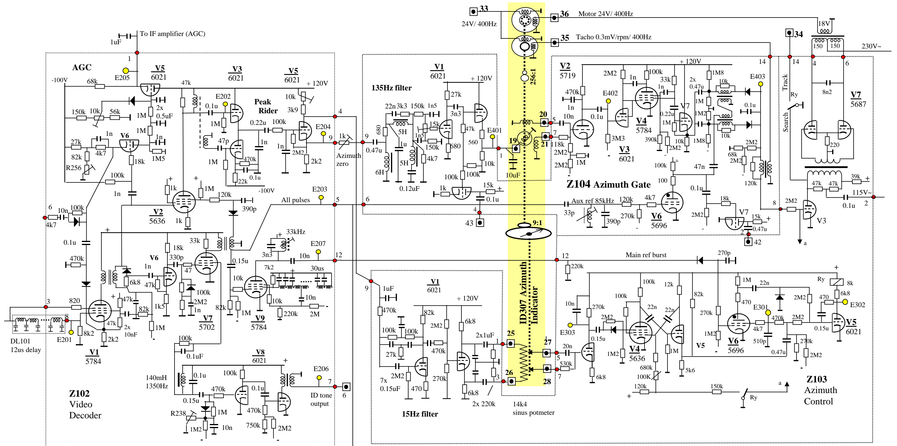
RT220C Video and Azimuth Circuit Diagram 9 feb 2008
